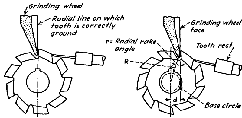
Figure 37B.--Form-relieved cutters are jace-sharpened only.
