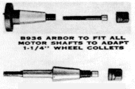
B936B ARBOR TO ADPAT B855, B955 QUILL FOR 1-1/4" WHEEL COLLETS
