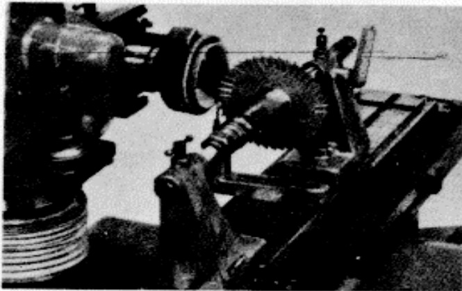
B827 Plain Micrometer Toothrest
