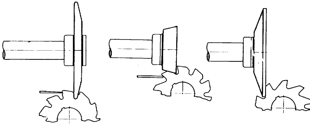
Figure 68B First Operation in Salvaging a Cutter.
