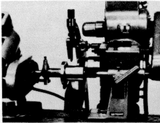
B6035 Coolant System
