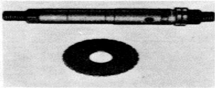
B648D INDEX DISCS 24 UP TO 60 DIVISIONS B948 SERIES CUTTER AND HOB GRINDING ARBORS
