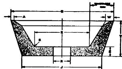
Type No. 11 Flaring Cup
