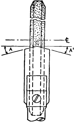
Figure 17.-Shape of blade of tooth rest for sharpening staggered tooth milling cutters.
