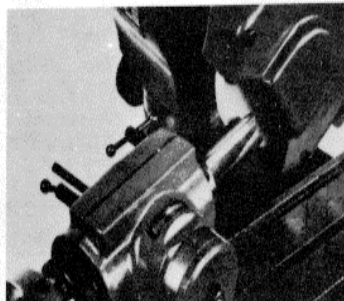
Sharpening a standard tap.
