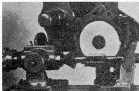
Sharpening a 2 1/2" tap.
