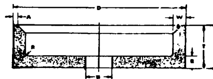
Type No. 6 Beveled Face
