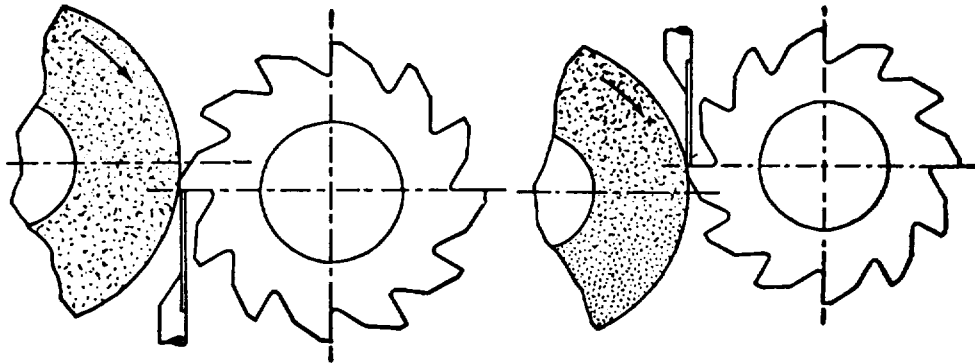
Figure 11.-Showing method of grinding with wheel rotating off cutting edge.
